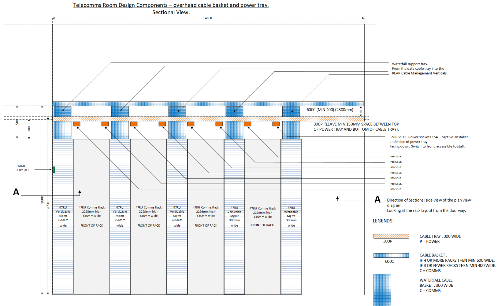
Figure 3 – 4-rack/cabinet room layout example. Side view.
