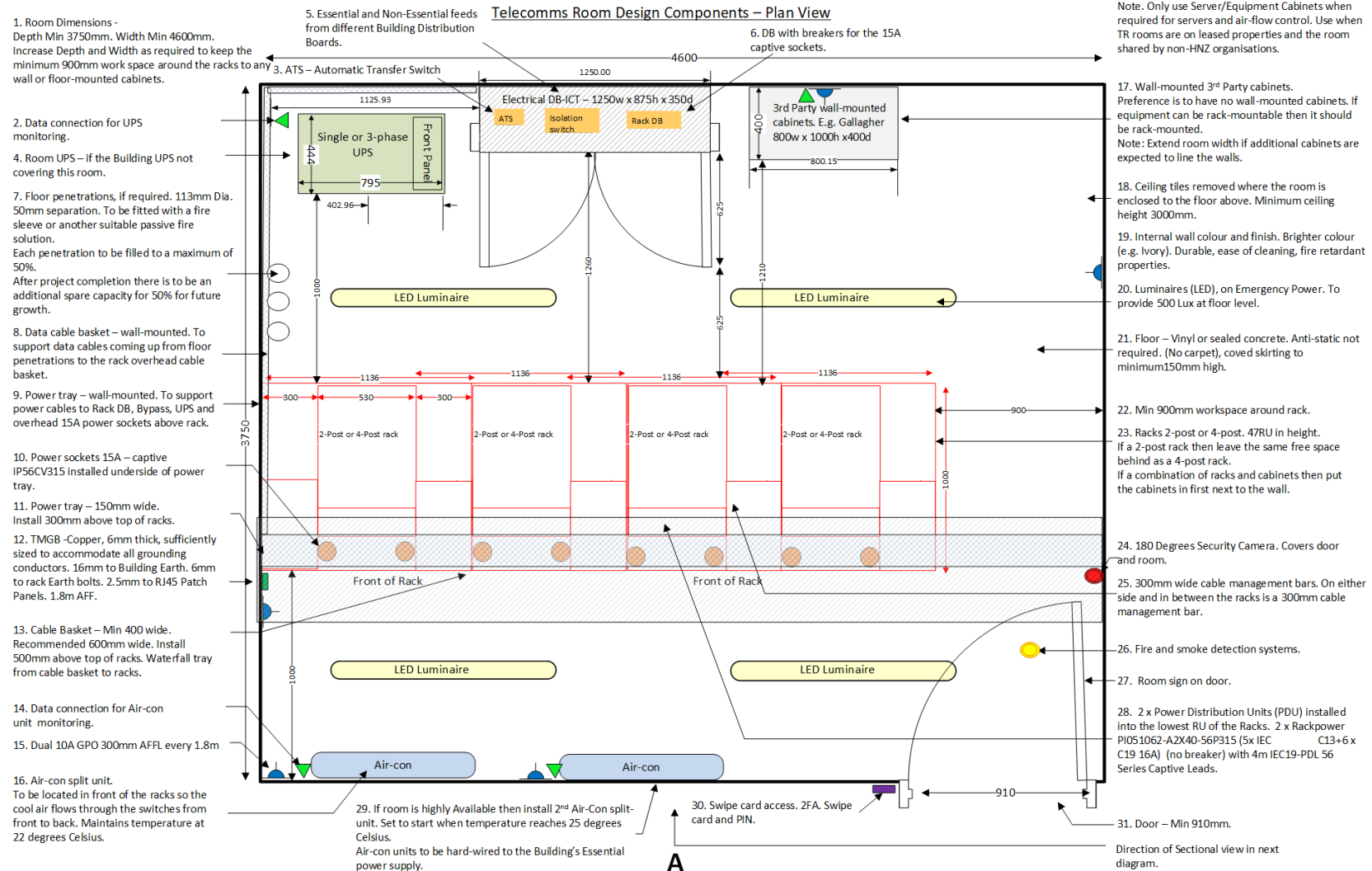
Figure 2 – 4-rack/cabinet room layout example.
