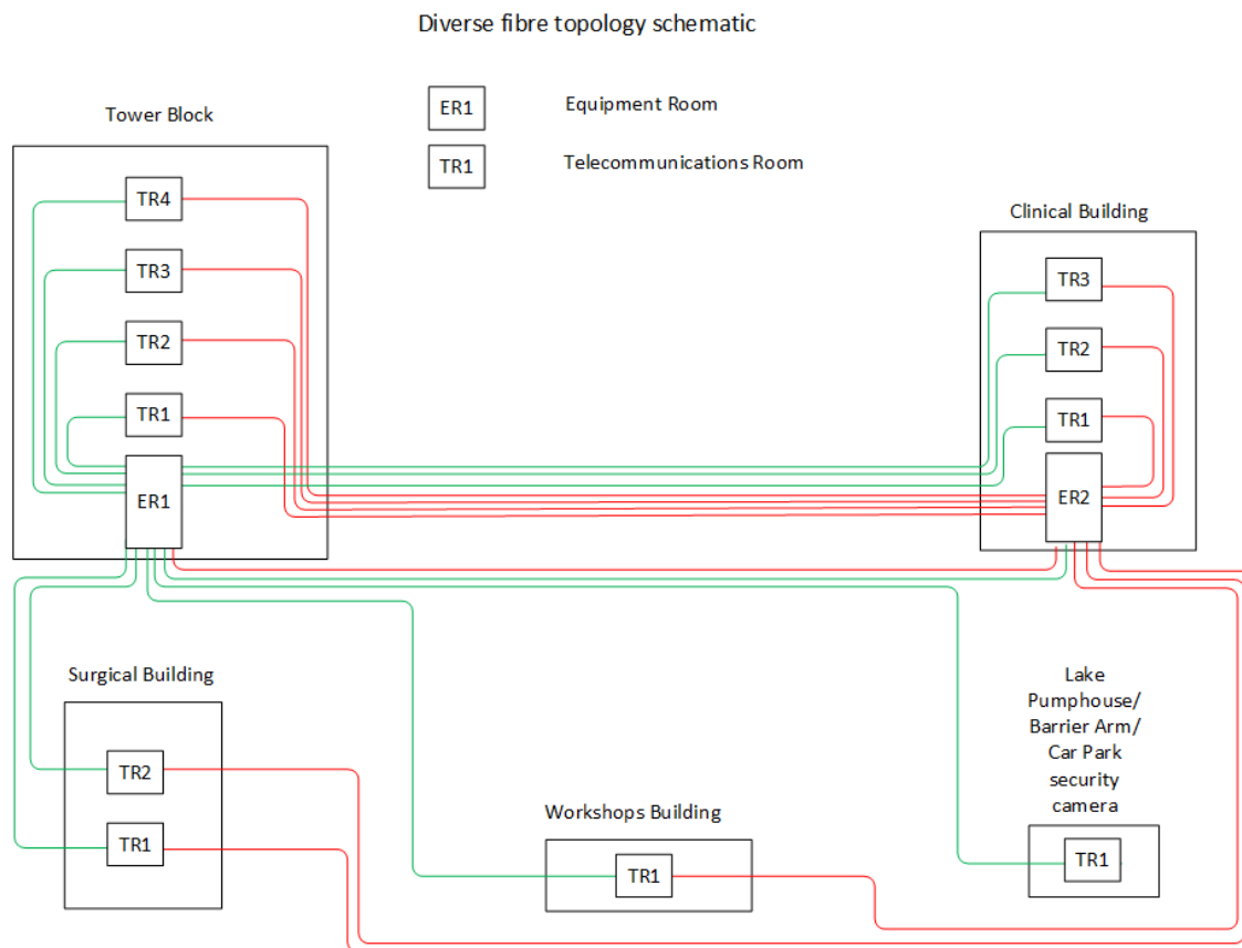
Figure 22 - Backbone topology #1, green (primary) and red (secondary) paths.
