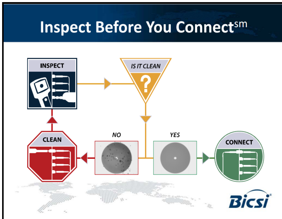
Figure 24 - Inspect Before You Connect
