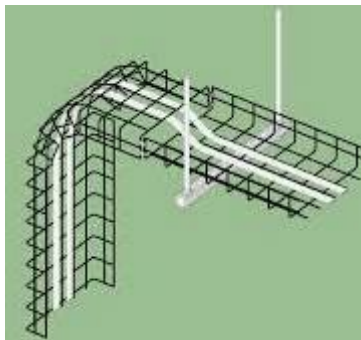
Figure 7 - waterfall cable basket example
