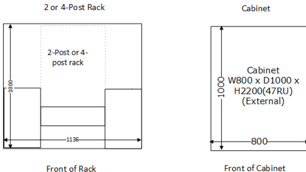
Figure 19 - Rack Dimensions example 3
