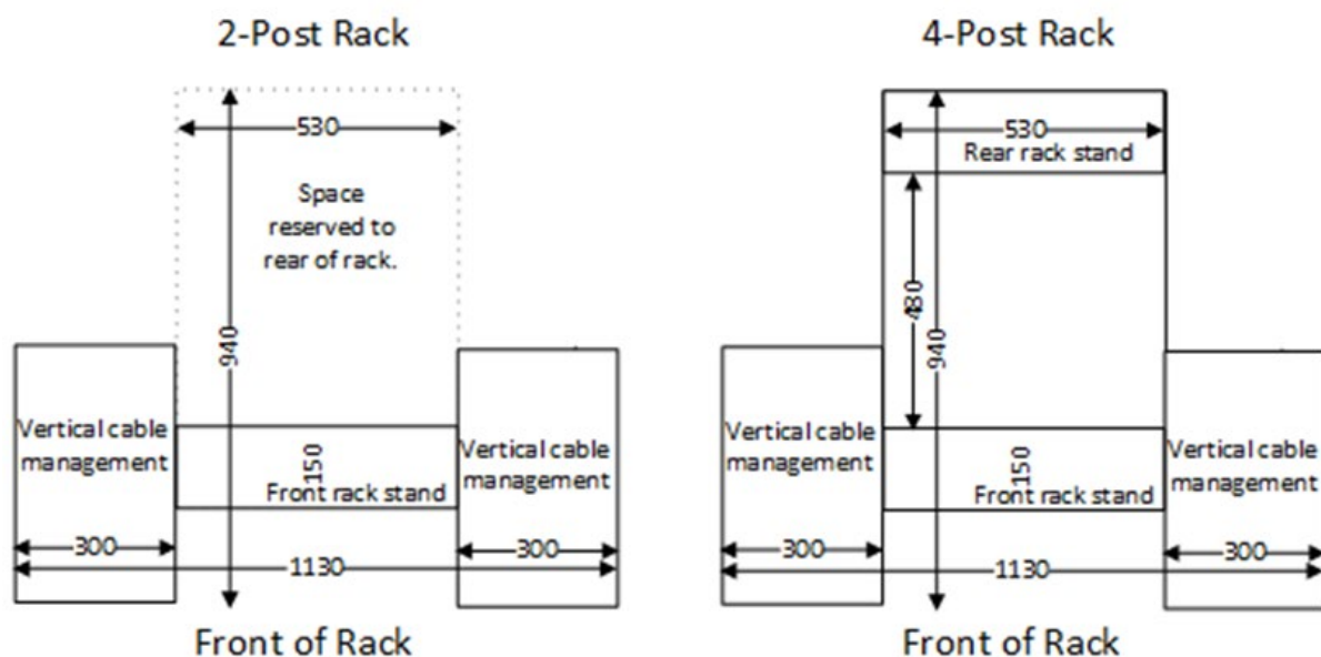
Figure 17 - Rack dimensions example 1
