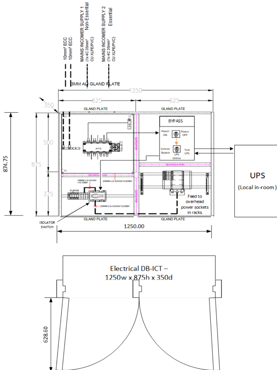
Figure 8 - Electrical DB, ATS, isolating switch. With a UPS in the room
