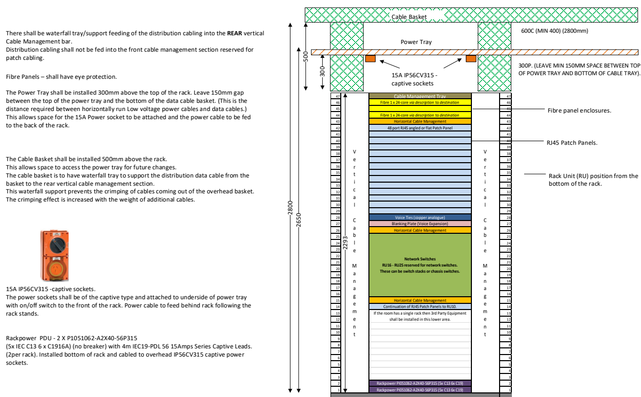
Figure 12 - Rack Layout – Patch Panels and Equipment
