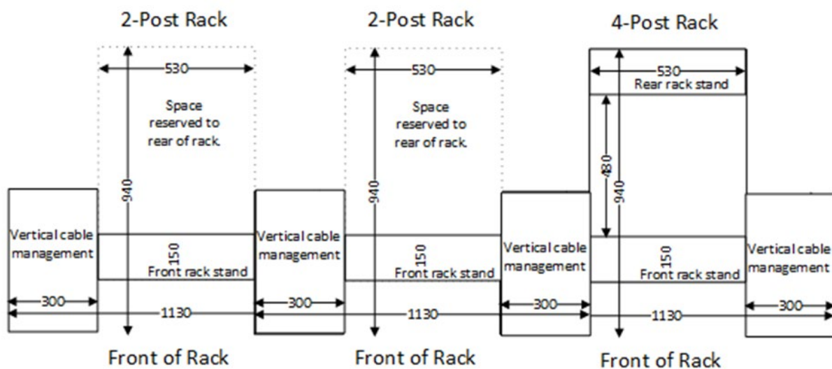
Figure 18 - Rack dimensions example 2
