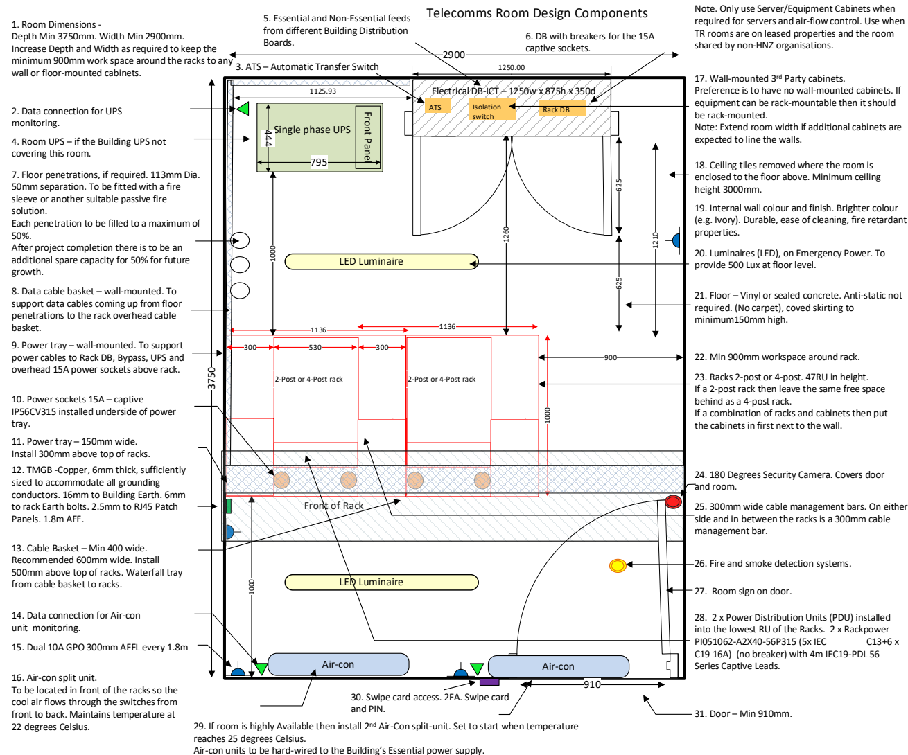
Figure 5 - 2-rack/cabinet room layout example.
