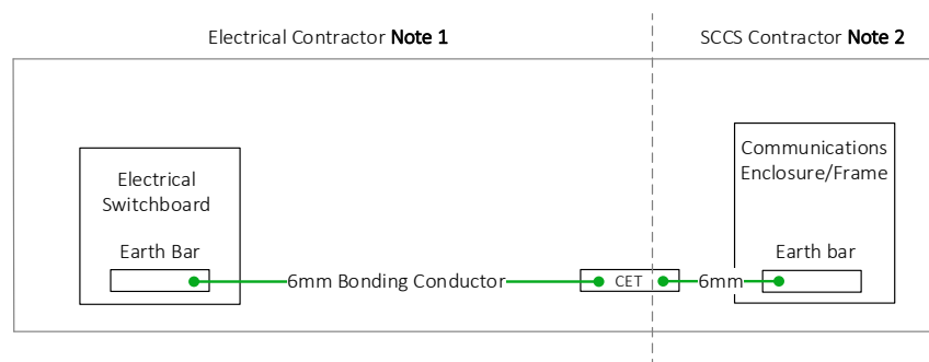
Figure 20 - Communications Earth Terminal responsibility
