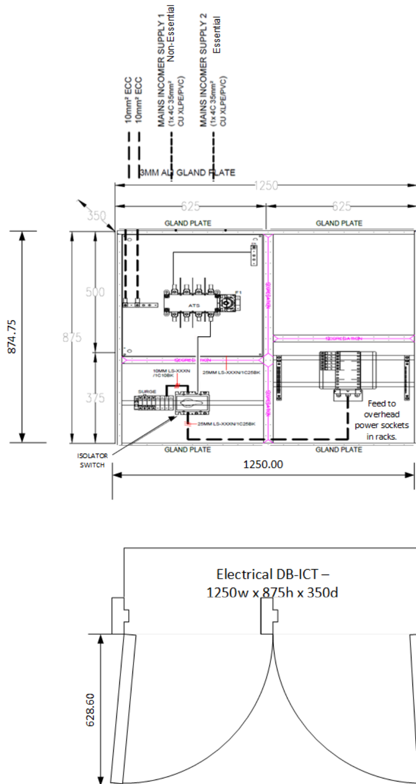
Figure 9 - Electrical DB, ATS, isolating switch. No UPS in the room.
