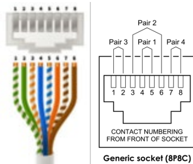
Figure 23 - T568A wiring pattern.
