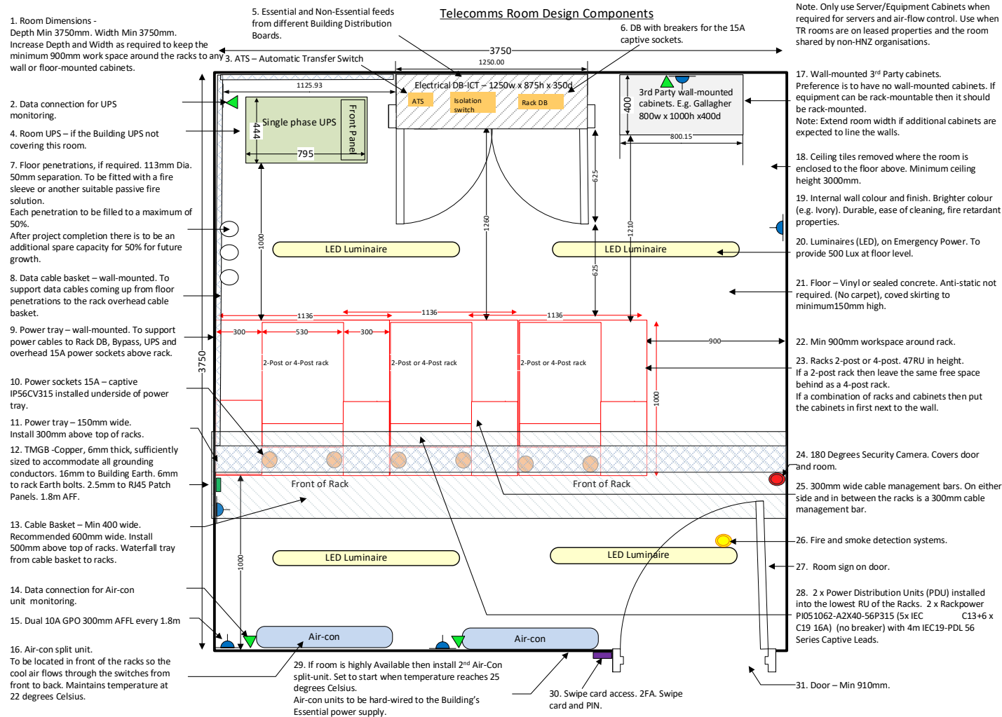
Figure 4 – 3-rack/cabinet room layout example.
