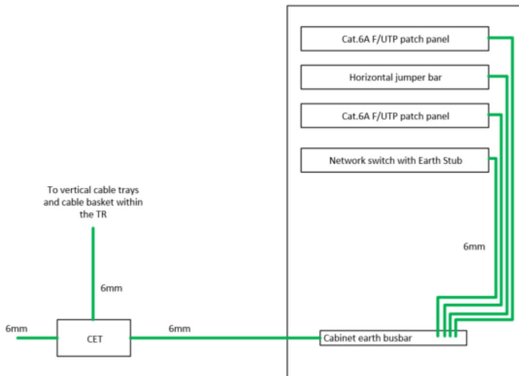
Figure 21 - Communications Earth Terminal structure
