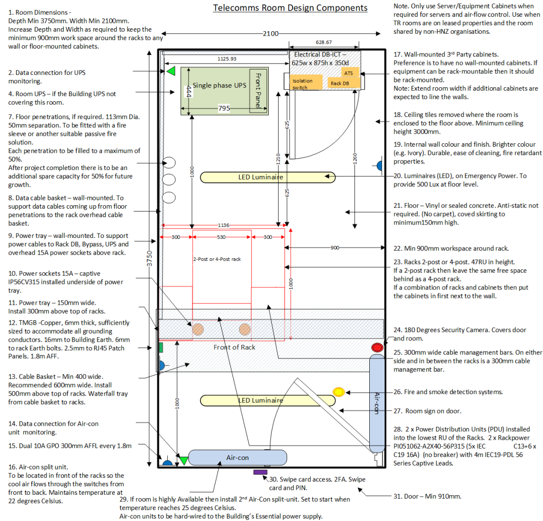
Figure 6 –1-rack/cabinet room layout example.
